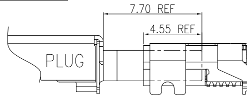
MATING INTERFACE
