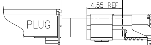
MATING INTERFACE
