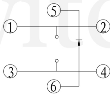
CIRCUIT
