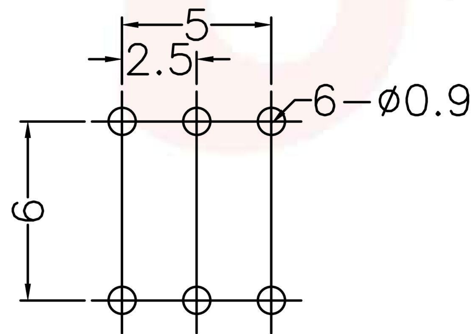
P.C.B LAYOUT BOTTOM VIEW
