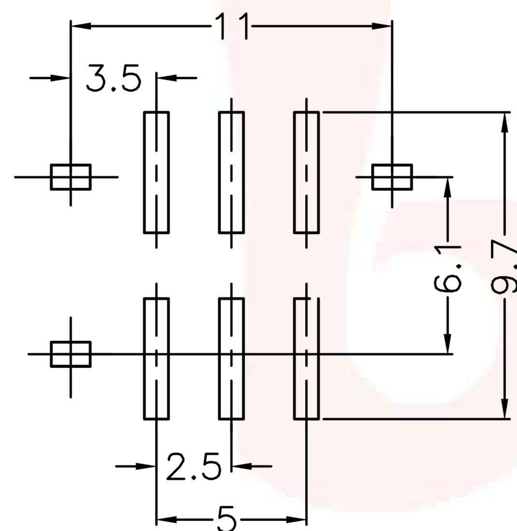
P.C.B LAYOUT BOTTOM VIEW
