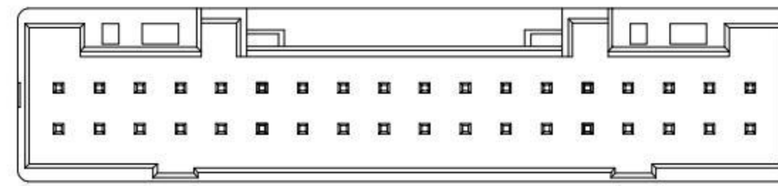
36Pin
