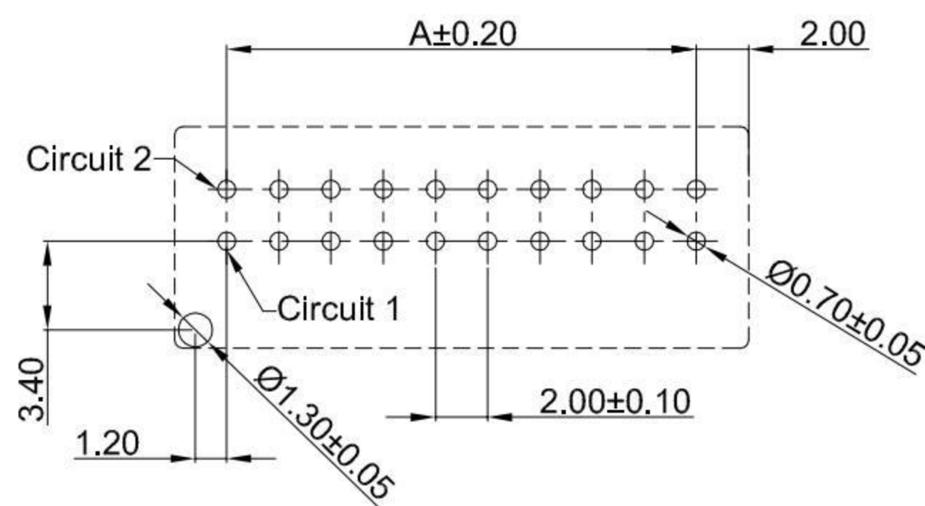
RECOMMENDED PCB LAYOUT TOLERANCE:±0.05
