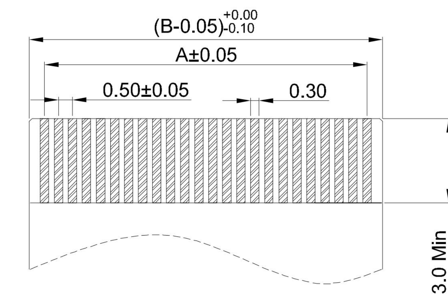
APPLICABLE FPC
