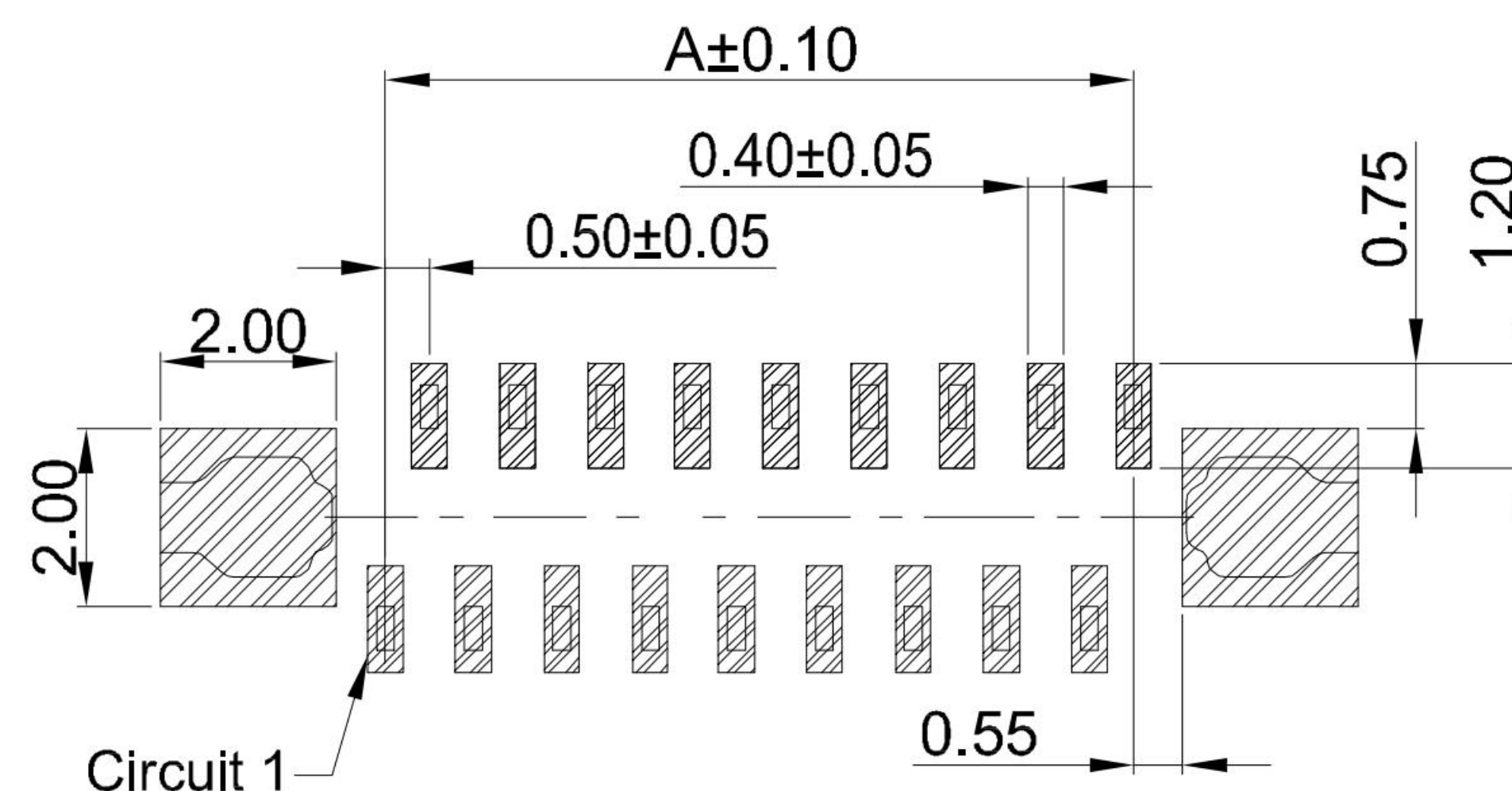
RECOMMENDED PCB LAYOUT TOLERANCE: \pm 0.05
