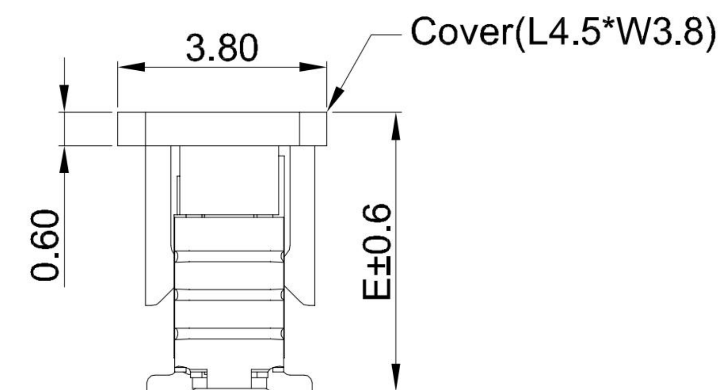
6PIN-60PIN WITH COVER
