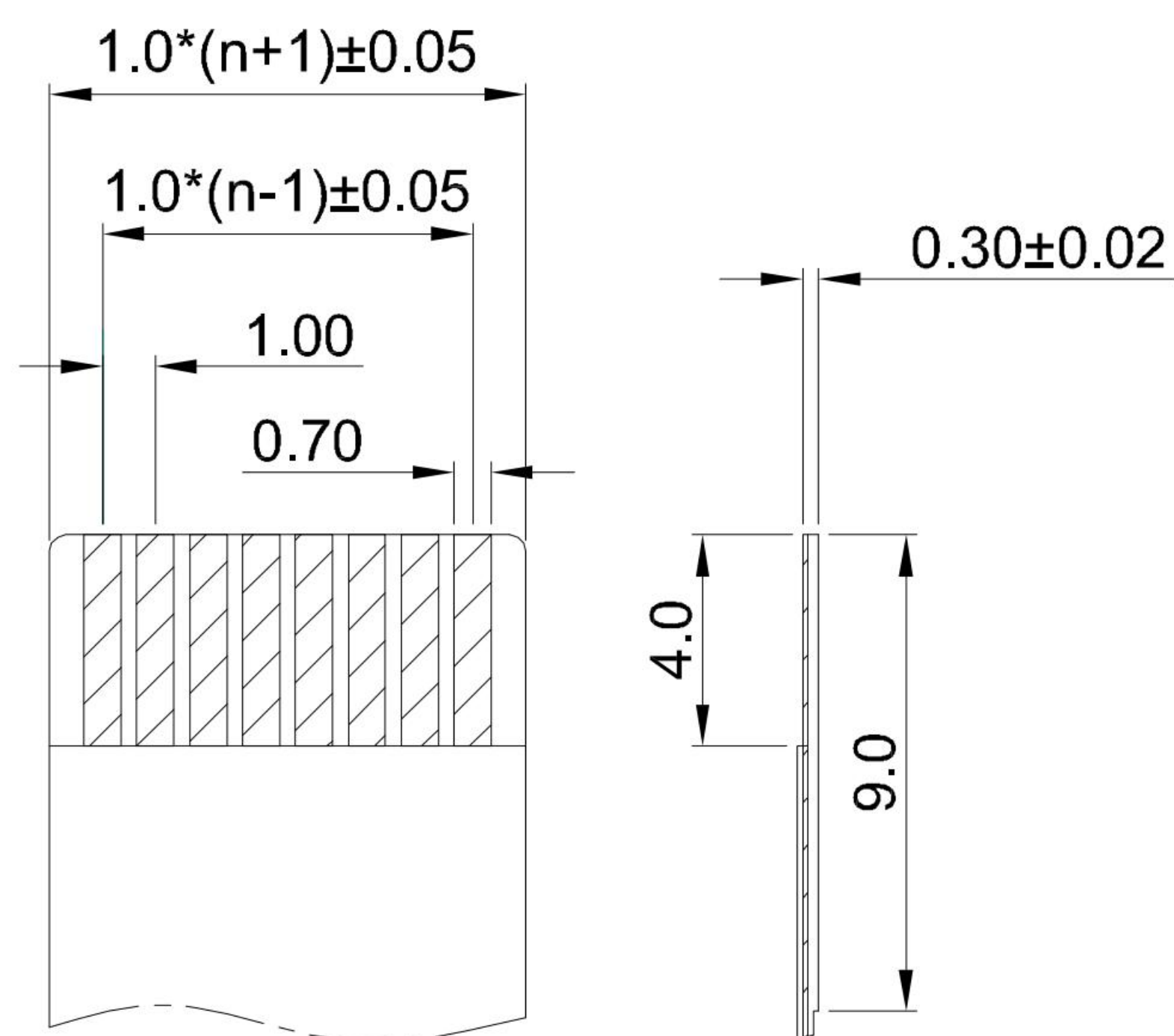
PROPER CABLE (SCALE 2:1)
