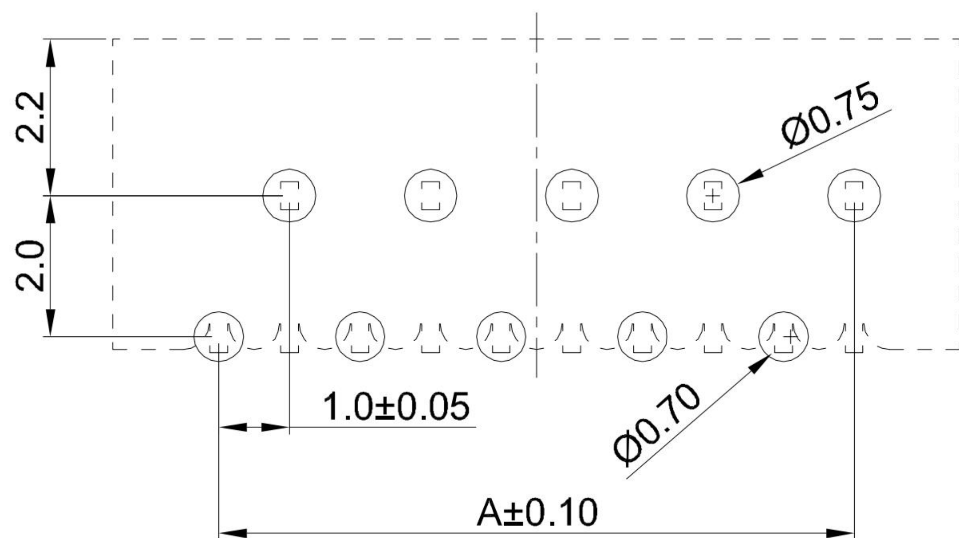
RECOMMENDED PCB LAYOUT TOLERANCE:±0.05
