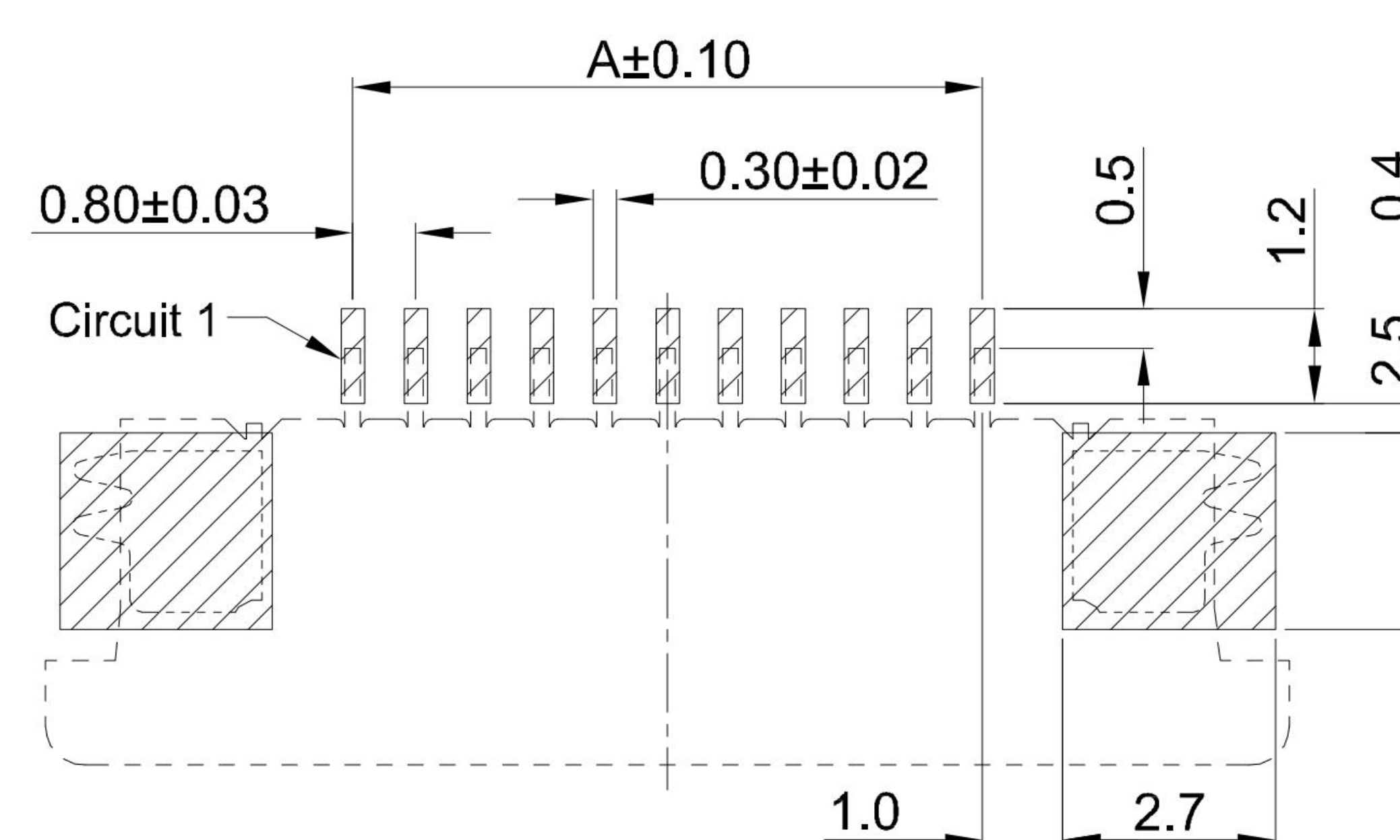
RECOMMENDED PCB LAYOUT TOLERANCE:±0.05
