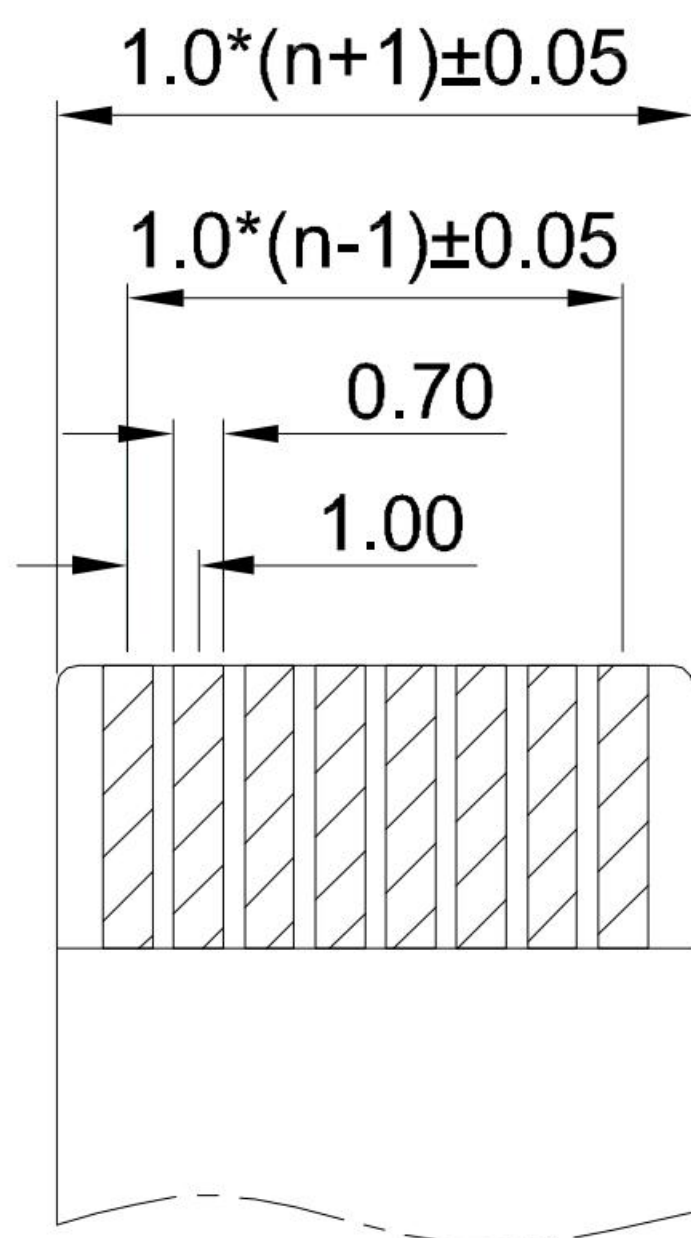
PROPER CABLE (SCALE 2:1)
