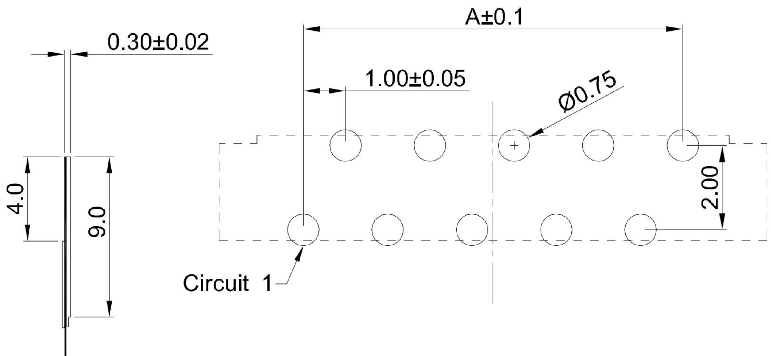
RECOMMENDED PCB LAYOUT TOLERANCE:±0.05
