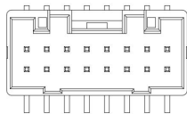
16Pin
