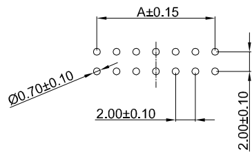
PCB REFERENCE DIAGRAM TOLERANCE:±0.05
