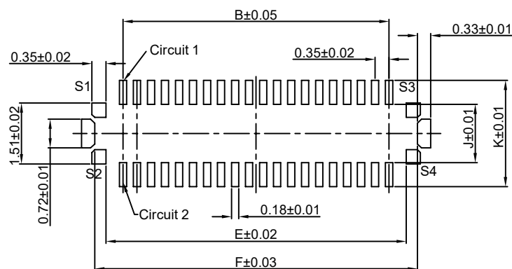
RECOMMENDED METAL MASK DIMENSIONS
