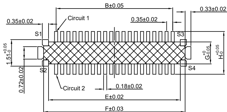
PCB REFERENCE DIAGRAM
