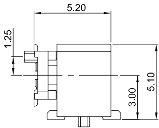
MATING HEIGHT
