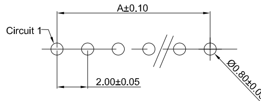
PCB REFERENCE DIAGRAM TOLERANCE:±0.05
