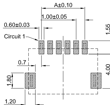
PCB REFERENCE DIAGRAM TOLERANCE:±0.05
