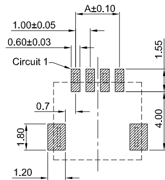
PCB REFERENCE DIAGRAM TOLERANCE:±0.05
