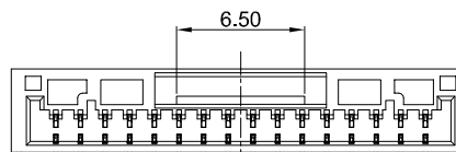
16Pin
