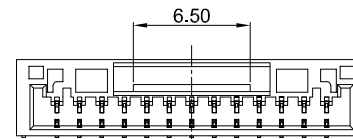
13Pin
