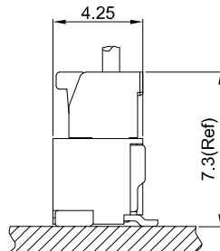
ASSEMBLY LAYOUT
