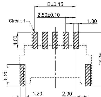
PCB REFERENCE DIAGRAM TOLERANCE: ±0.05
