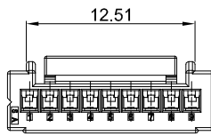
9PIN
