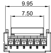
6PIN
