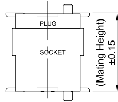
MATING HEIGHT
