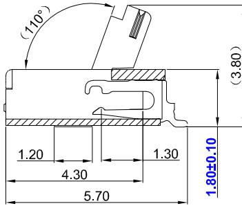
SECTION A-A(2:1)
