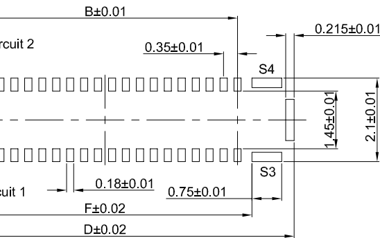
RECOMMENDED METAL MASK DIMENSIONS METAL MASK THICKNESS: 80um
