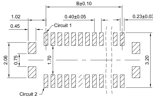
PCB REFERENCE DIAGRAM TOLERANCE:±0.05
