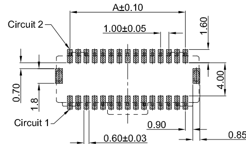
PCB REFERENCE DIAGRAM TOLERANCE:±0.05
