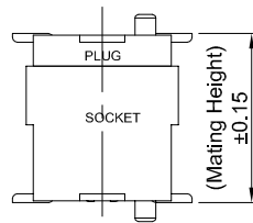
MATING HEIGHT
