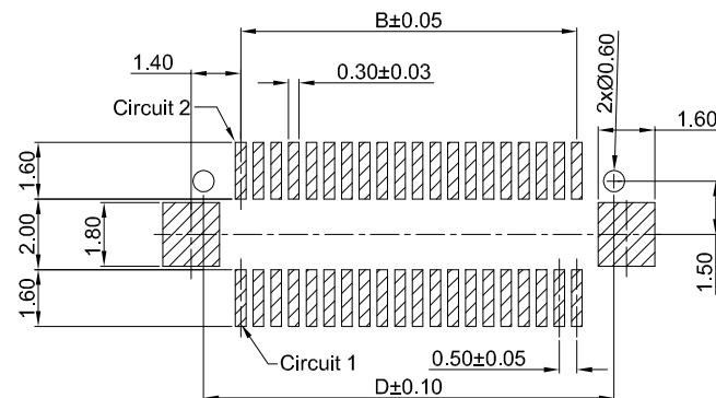
PCB REFERENCE DIAGRAM TOLERANCE:±0.05
