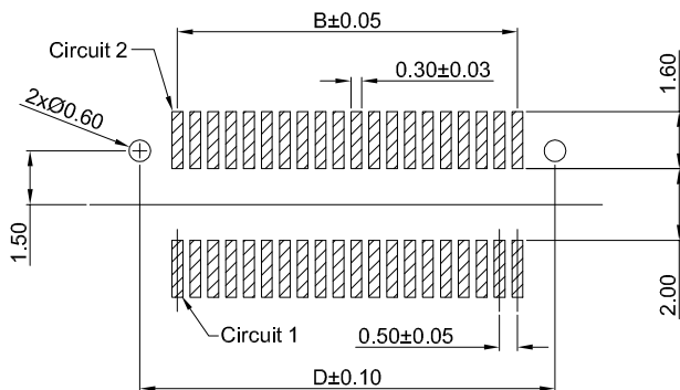
PCB REFERENCE DIAGRAM TOLERANCE:±0.05
