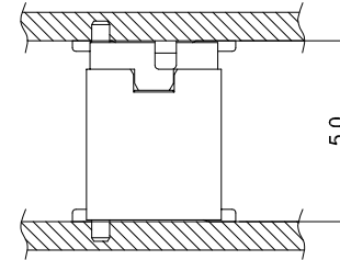
MATING HEIGHT
