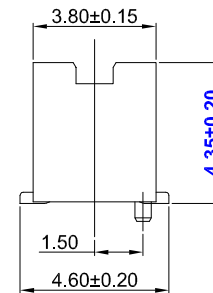
MATING HEIGHT
