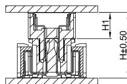
MATING HEIGHT
