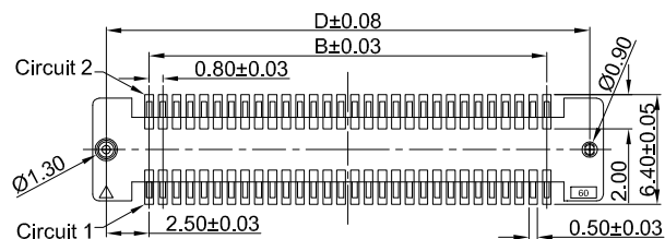
PCB REFERENCE DIAGRAM TOLERANCE:±0.05
