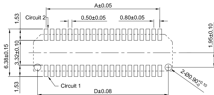
PCB REFERENCE DIAGRAM TOLERANCE:±0.05
