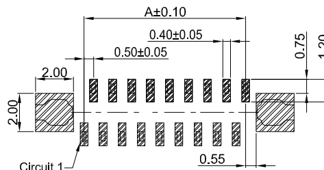
PCB REFERENCE DIAGRAM TOLERANCE:±0.05
