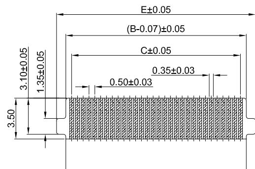
APPLICABLE FPC
