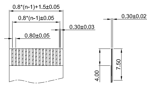
APPLICABLE FPC
