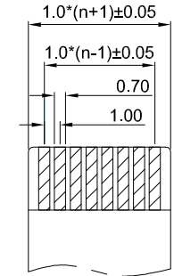
PROPER CABLE (SCALE 2:1)
