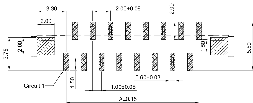
PCB REFERENCE DIAGRAM TOLERANCE:±0.05
