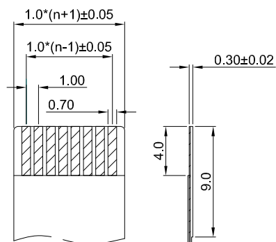
PROPER CABLE (SCALE 2:1)
