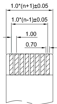
PROPER CABLE (SCALE 2:1)
