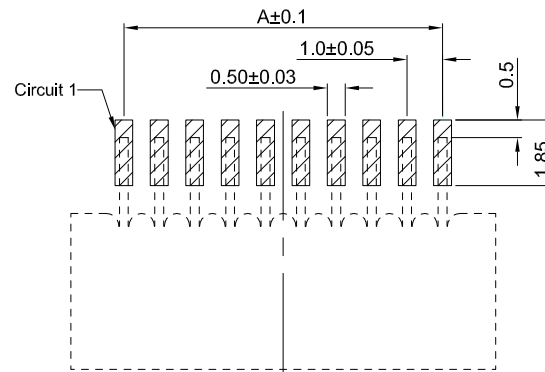
PCB REFERENCE DIAGRAM TOLERANCE:±0.05
