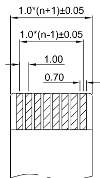
PROPER CABLE (SCALE 2:1)
