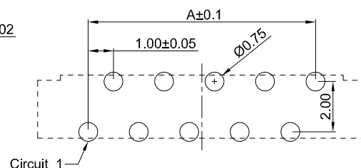
PCB REFERENCE DIAGRAM TOLERANCE:±0.05
