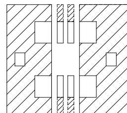
PCB REFERENCE DIAGRAM TOLERANCE:±0.05
