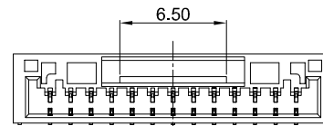
13Pin
