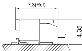
ASSEMBLY LAYOUT
