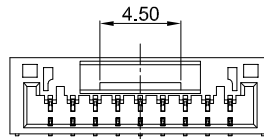
9Pin
