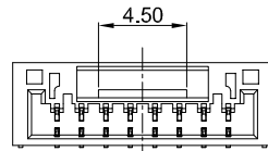
8Pin
