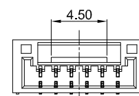
6Pin
