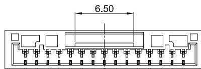
15Pin
