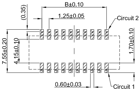
PCB REFERENCE DIAGRAM TOLERANCE:±0.05
