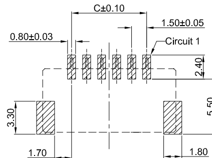
PCB REFERENCE DIAGRAM TOLERANCE:±0.05
