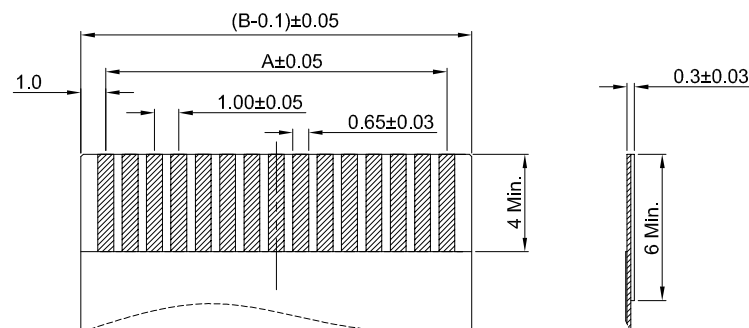
APPLICABLE FLAT CABLE
